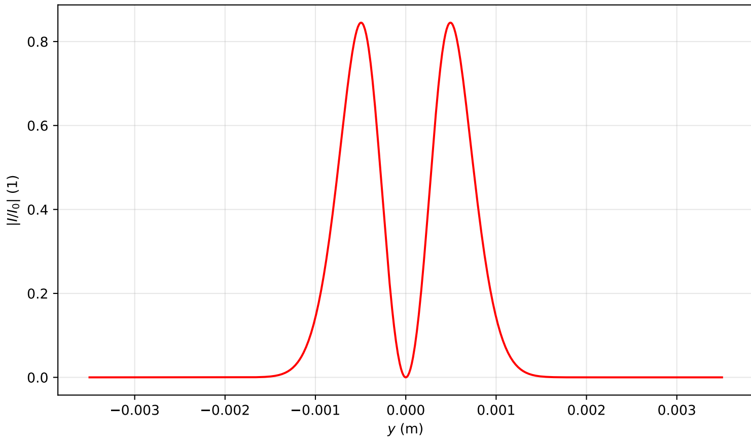
Intensity profile I(x=0, y, z=0.159)/I_0 , P_{in}=4.0P_{cr} , artificial time
